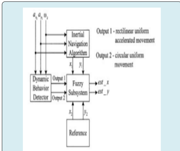
Figure 8: Schematics of fuzzy integrated navigation system.
