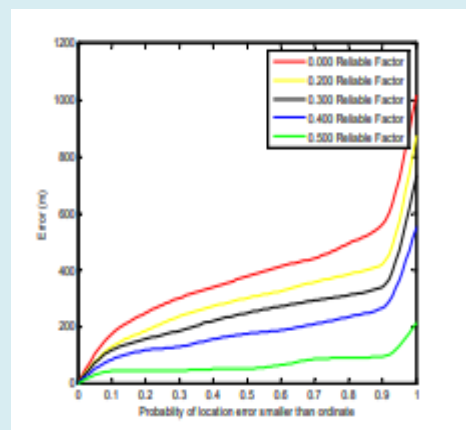
Figure 7: Performance comparisons for different Reliable Factor.
