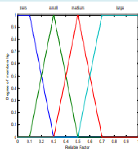
Figure 6: Membership function of Reliable Factor.
