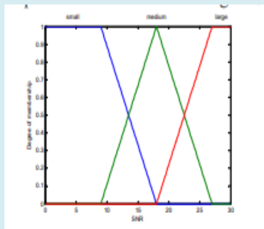
Figure 5: Membership function of SNR.
