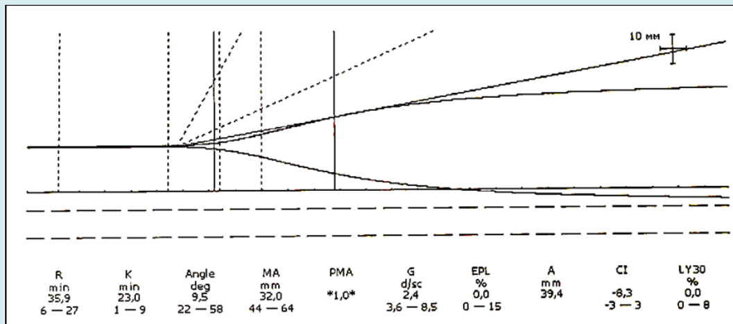
Figure 3: Clinical example of the development of the hypocoagulable phase of DIC on TEG (Platelets - 218 \times 10^9/L ; Hb - 129 \text{ g/L} ; Fibrinogen - 4.54 \text{ g/L} ; D-Dimer - 2500 \mu\text{g/L} ).
