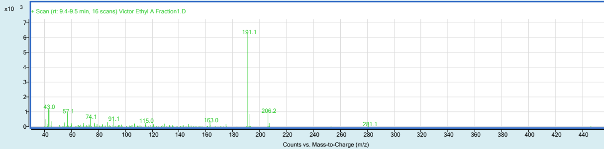
Figure 8: Phenol, 2,5-Bis(1,1-Dimethylethyl).
