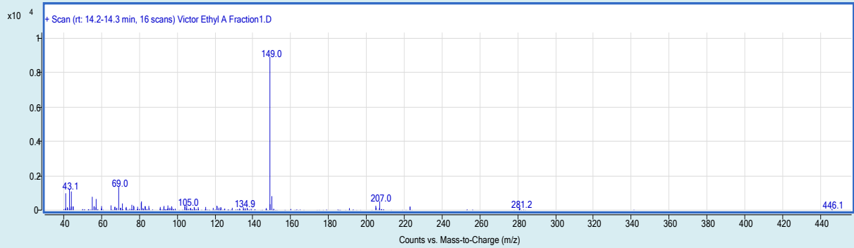
Figure 5: Dibutyl phthalate.
