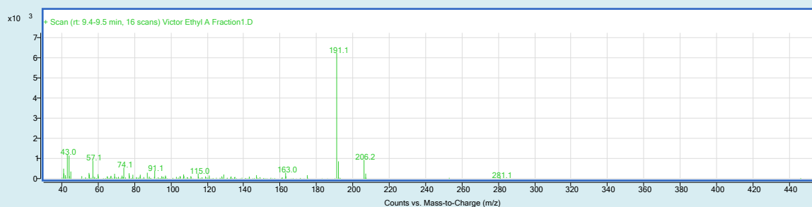
Figure 10: Benzenepropanoic Acid, 3,5-Bis(1,1-Dimethylethyl)-4-Hydroxy-, Methyl Ester.
