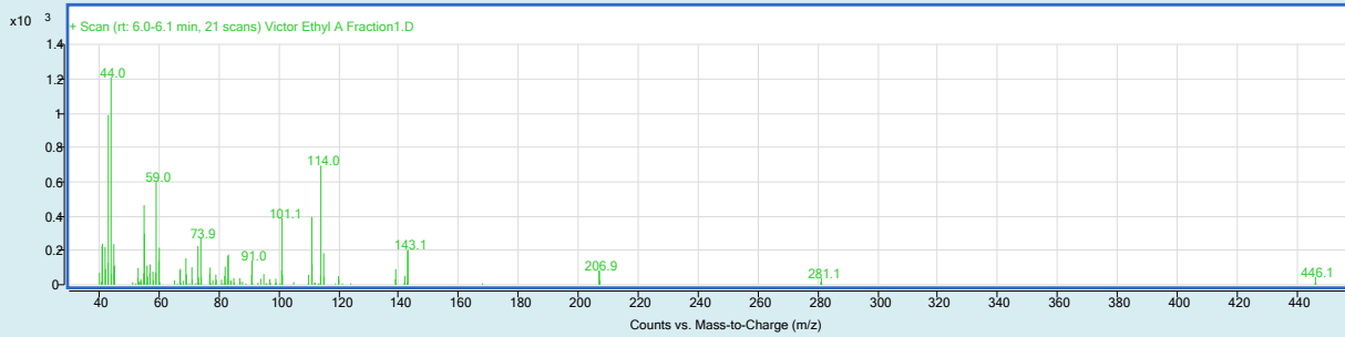
Figure 6: Hexadecanoic Acid, Methyl Ester.
