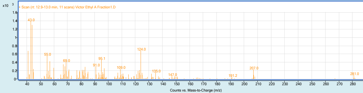
Figure 7: 2-Methyl-3-(3-Methyl-But-2-Enyl)-2-(4-Methyl-Pent-3-Enyl)-oxetane.
