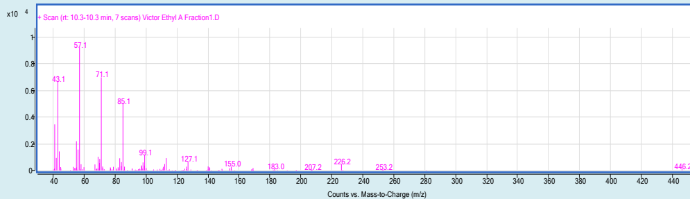
Figure 3: 2-Decanol.
