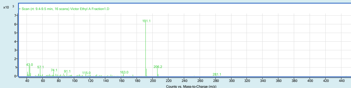
Figure 9: Pentanoic Acid, 5-Hydroxy-, 2,4-Di-T-Butylphenyl Esters.
