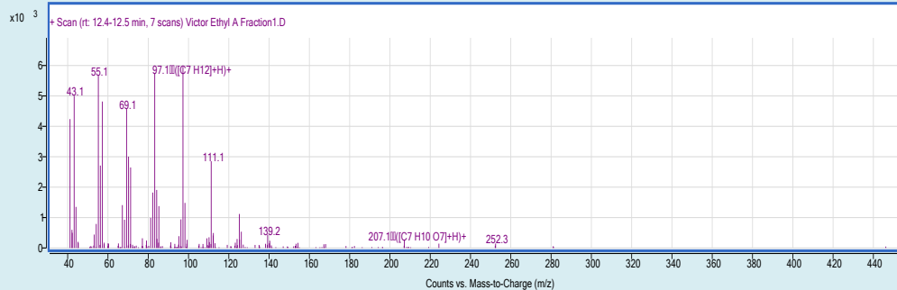
Figure 4: Phytol.
