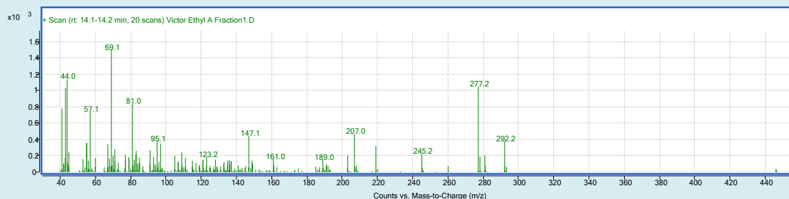
Figure 11: Ethanethoic Acid, S-(4-Methylphenyl) Ester.
