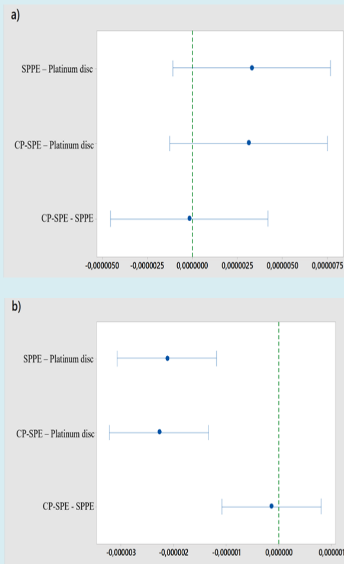
Appendix 1: Graphs Related to the Tukey Test for Comparing the Means of Concentrations Obtained with Platinum CP-SPE, Disk Electrodes and SPPE for \Delta 9 -THC (A) and CBD (B) with a 95% Confidence Interval.
