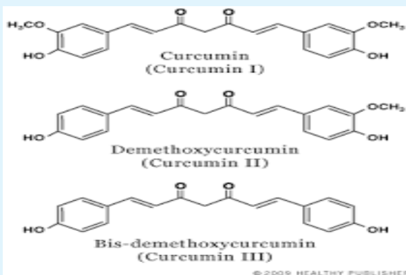
Figure 6: Curcuminoids.
