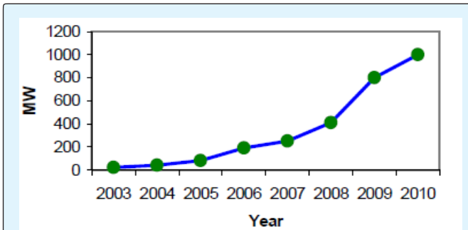
Figure 4: Average windfarm capacity 2003-2010 (Mega watts, MW).
