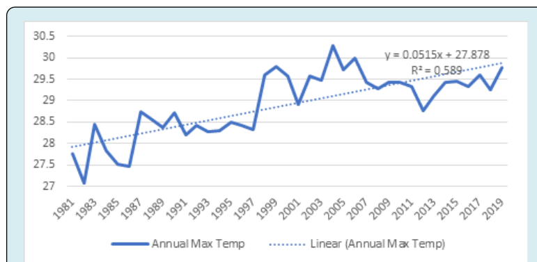
Figure 10: Trend in Max. Temperature at Gembu.
