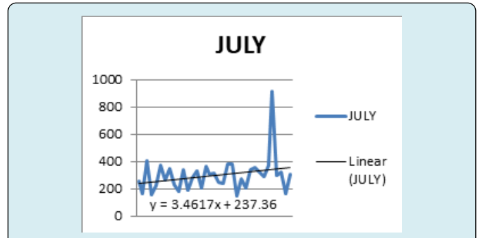
Figure 7: July Rainfall in Gembu.
