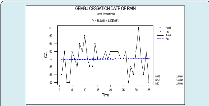
Figure 4: Trend of Cessation Dates of Rain in Gembu.
