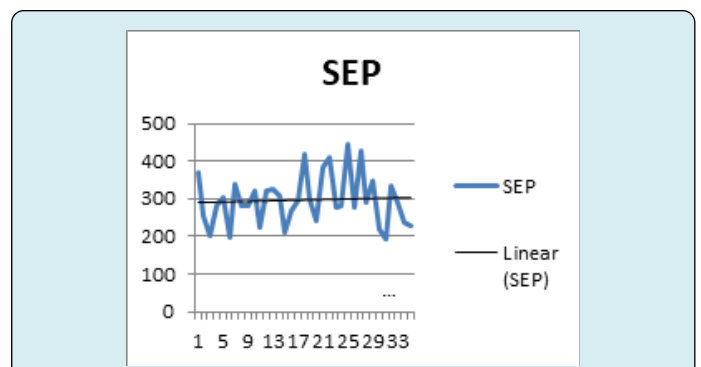
Figure 9: September Rainfall in Gembu.
