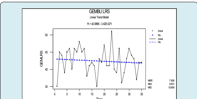
Figure 6: Trend of Length of Rainy Season in Gembu.
