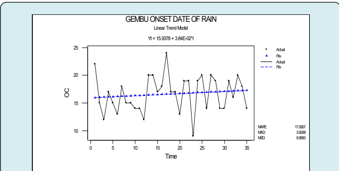
Figure 5: Trend of Onset Date of Rainfall in Gembu.
