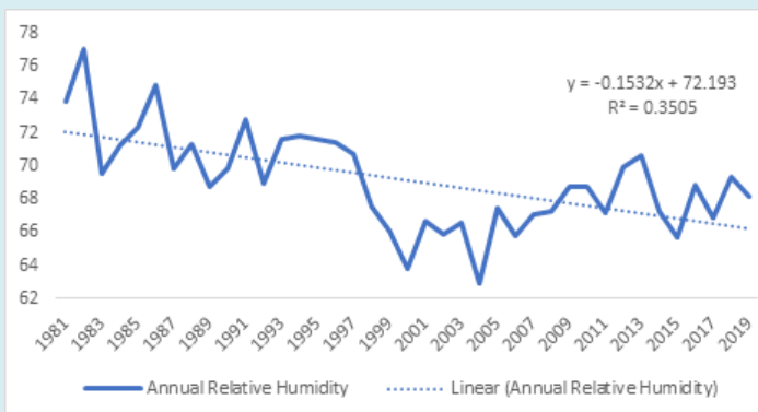
Figure 14: Trend in Relative Humidity at Gembu.
