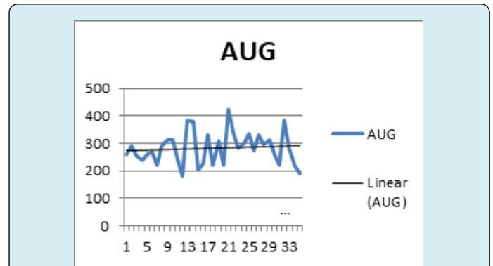
Figure 8: August Rainfall in Gembu.
