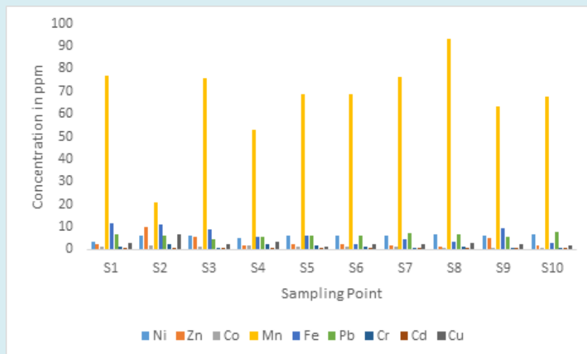
Figure 5: Distribution of Heavy Metal in the Carbonate Phase with Respect to Sampling Points.
