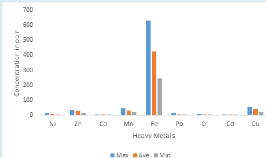
Figure 10: Organic Phase with respect Maximum, Average and Minimum Concentration.
