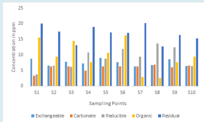
Figure 13: Concentration of (Ni) in Respect to Sampling Point and Phases.
