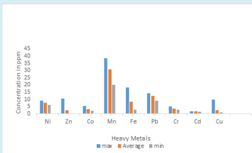
Figure 4: Exchangeable Phase with respect to minimum, average and maximum concentration of metals along the sampling points.
