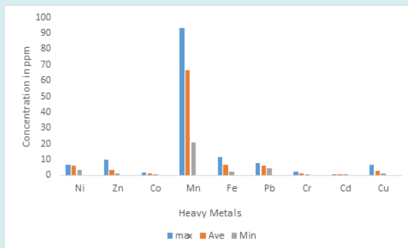
Figure 6: Bar chart showing the Carbonate Phase with respect to Maximum, average and Minimum of Heavy Metals Concentration.
