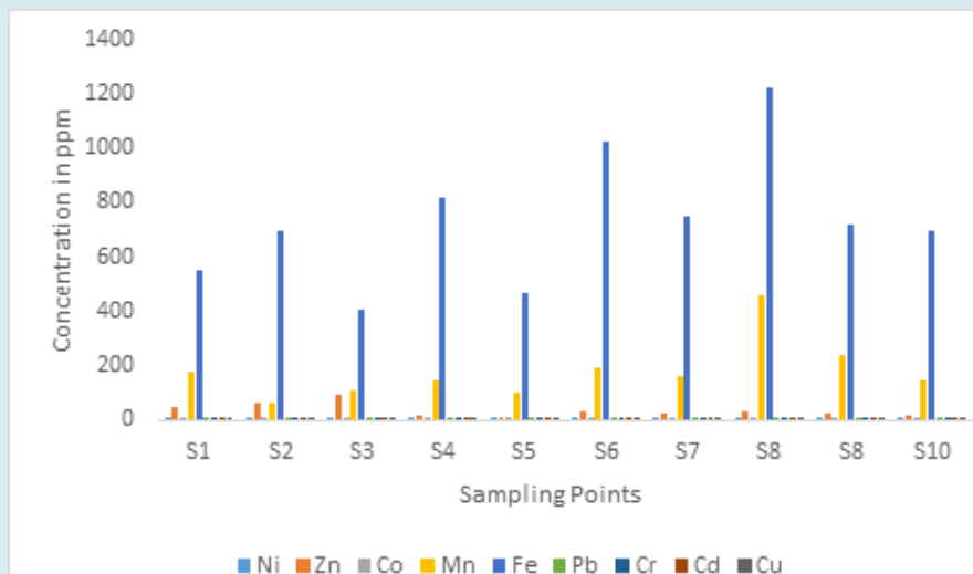
Figure 7: Distribution of Heavy Metals in Reducible Phase with Respect to Sampling Points.
