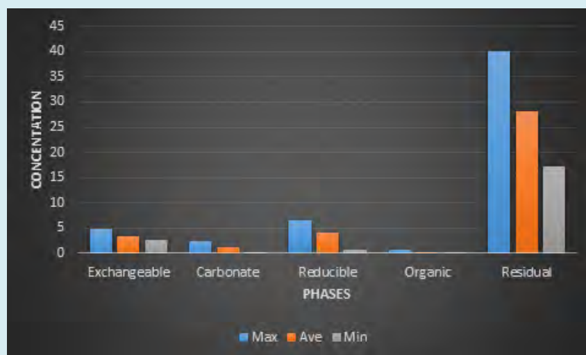
Figure 26: Maximum, Average and Minimum Concentration of Cr with respect to the mineralogical Phases.
