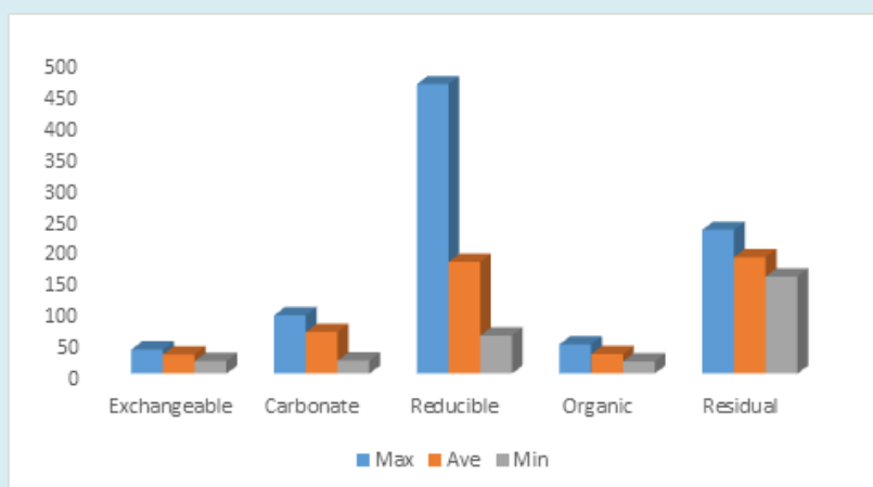
Figure 20: Maximum, Average and Minimum Concentration of Mn over all the Phases.
