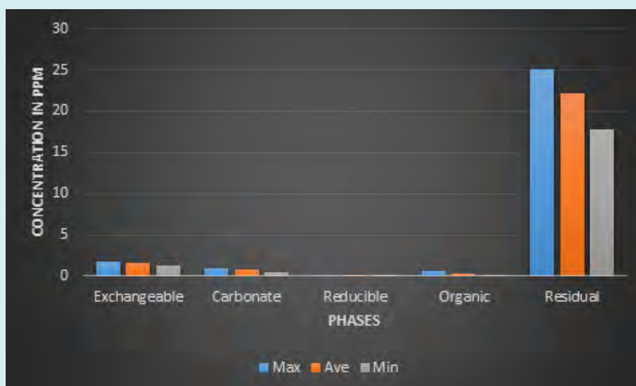
Figure 28: Maximum, Average and Minimum Concentration of Cd with respect to mineralogical Phases.
