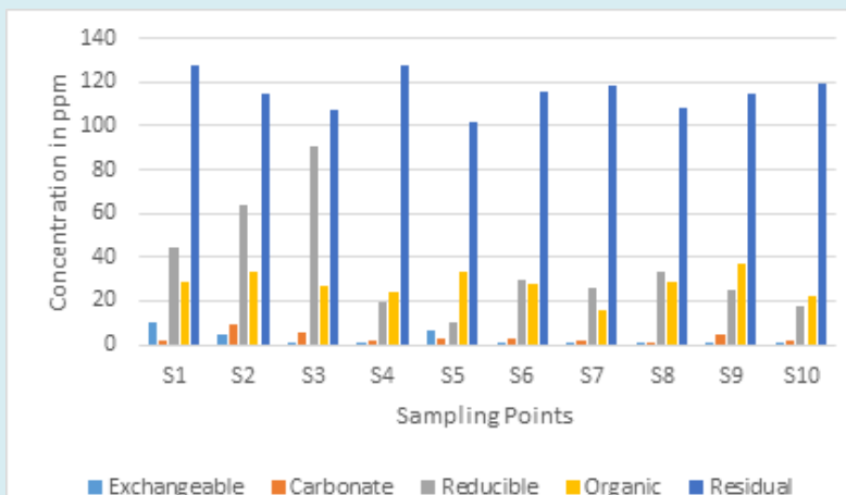
Figure 15: Concentration of (Zn) in Respect to Sampling Point and Phases.
