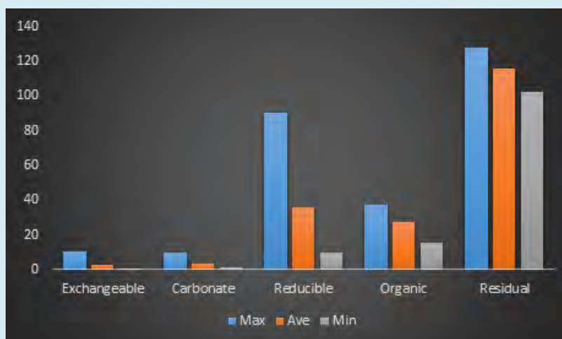
Figure 16: Maximum, average and minimum concentration of zinc with respect all the Phases.
