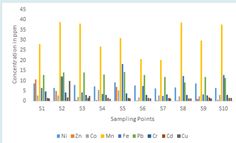
Figure 3: Distribution of Heavy Metal in the Exchangeable Phase with Respect to Sampling Points.
