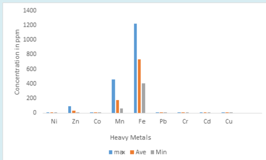
Figure 8: Bar chart showing distribution of heavy metals in Reducible phase.
