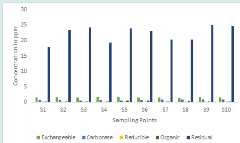
Figure 19: Concentration of (Mn) in Respect to Sampling Point and Phases.
