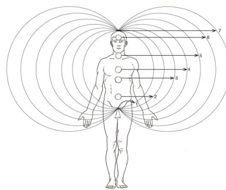
Figure 1: The 6+1 spinning energy centers and their discrete energy levels.
