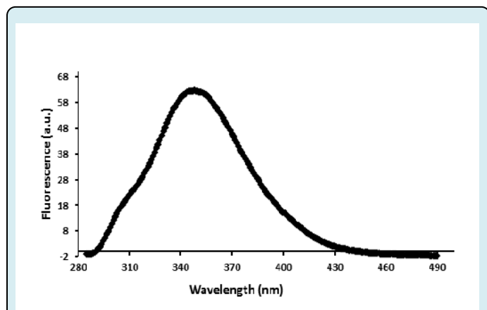
Figure 2: Plot of fluorescence emission of Libyan Cobra ( Naja haje ) venom (30µg/ml) vs wavelength from 285-490 nm using excitation of \lambda 280 nm in 0.01 M Tris, 0.1 M NaCl at pH 7.4. Spectra were corrected for small background fluorescence contributions from the buffer solution and were scaled to visualize the shift. (a.u: arbitrary units).
