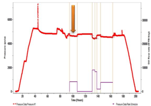
Figure 9: The first draw-down period.
