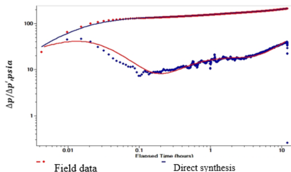
Figure 15: Direct synthesis model.
