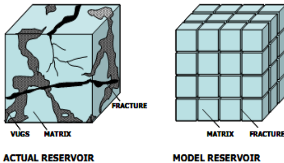
Figure 2: Ideal model for a natural fractured reservoir (after Warren and Root [10]).
