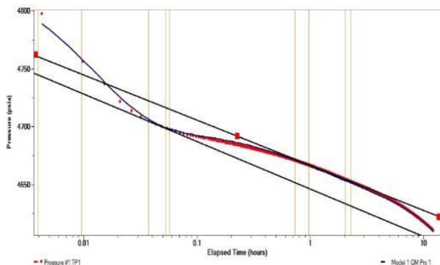
Figure 11: Conventional semi log plot.
