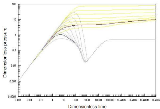
Figure 6: Derivative type curve for double-porosity reservoir, pseudo-steady state flow.
