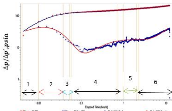
Figure 14: Typical pressure derivative and its periods.
