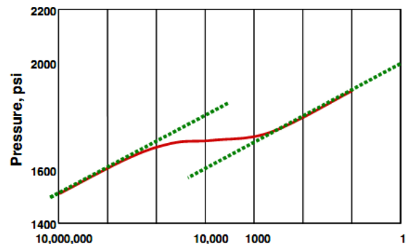
Figure 3: Semi log plot for pressure response in NFR.
