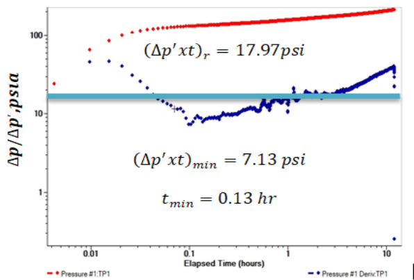
Figure 12: Pressure difference and its derivative plot.
