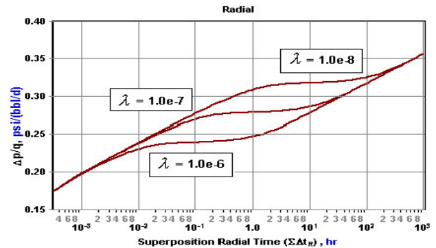
Figure 5: Effect of Interporosity on the pressure response with pseudosteady state interporosity flow. \omega = 0.01 .
