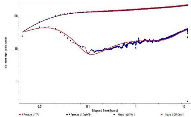
Figure 10: log-log plot of pressure difference and its derivative versus time.
