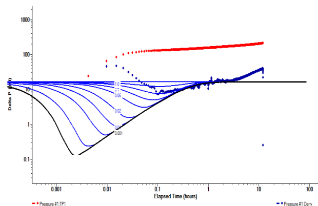
Figure 13: Type curve analysis.
