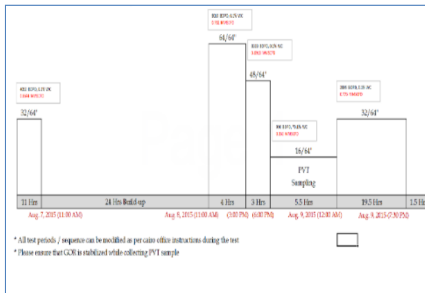
Figure 8: Rate schedule history used in test.
