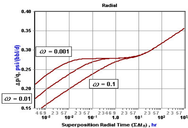
Figure 4: Effect of storativity ratio on the pressure response with pseudosteady state Interporosity flow. \lambda = 10^{-7} .
