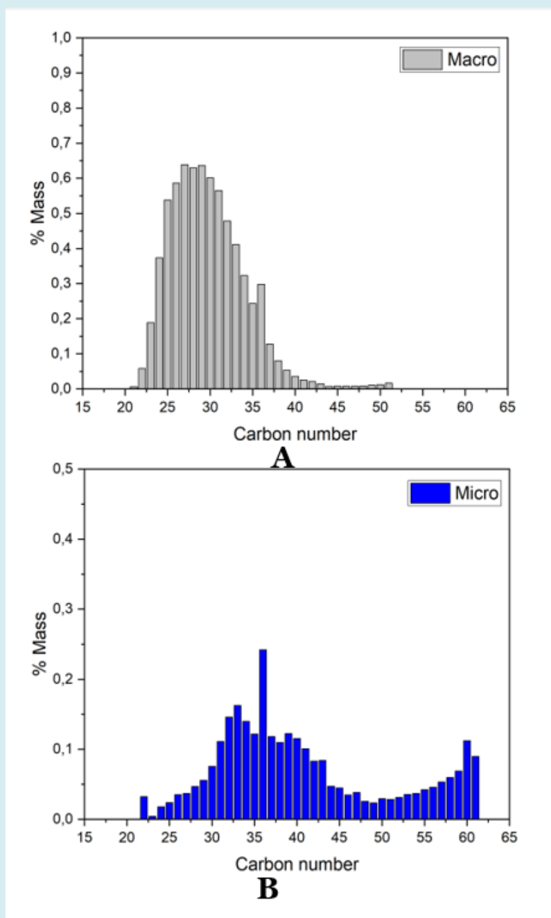
Figure S1: (A) Macrowax containing hydrocarbons with carbon numbers ranging from 21 to 51; (B) Microwax containing hydrocarbons with carbon numbers ranging from 22 to 61.
