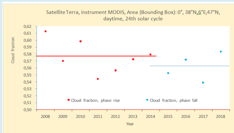
Figure 19: Daytime cloudiness over the western Mediterranean is about 1.5% more during the phase "rise" of the solar cycle than during the phase "fall".
