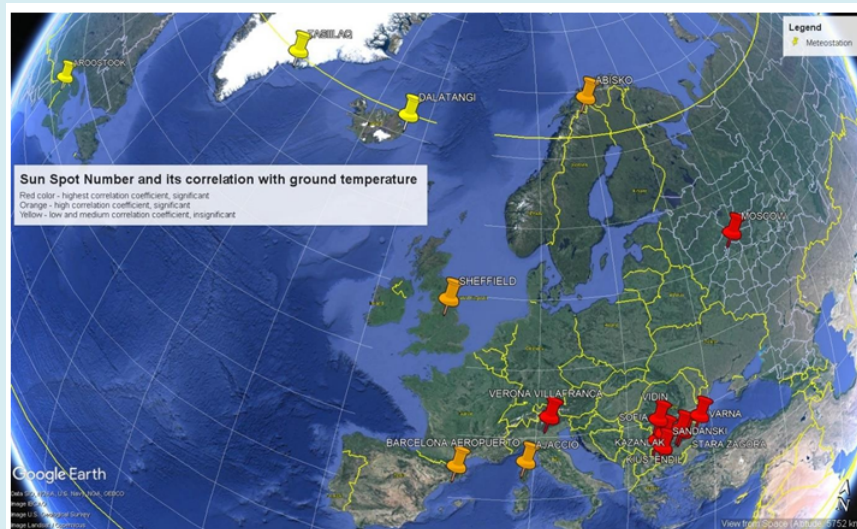
Figure 18: Google Earth map with stations from the Northern Hemisphere, the markers for which are colored depending on the magnitude of the correlation coefficient between surface air temperature and SSN for the phase “rise” of the solar cycles. With red color – a very high statistically significant correlation; with orange color high statistically significant correlation, with yellow color – a statistically insignificant correlation.
