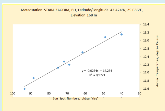
Figure 4: There is a linear relationship with a very high coefficient of determination between surface air temperature in the region of STARA ZAGORA, BULGARIA, and the number of sunspots, both calculated for the phase “rise” of the solar cycles included in the study.
