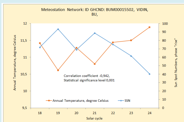
Figure 5: There is a high statistically significant negative correlation between the mean surface air temperature for the weather station VIDIN, BULGARIA, and the mean value of the number of sunspots during the phase “rise” of the last 7 cycles of solar activity.
