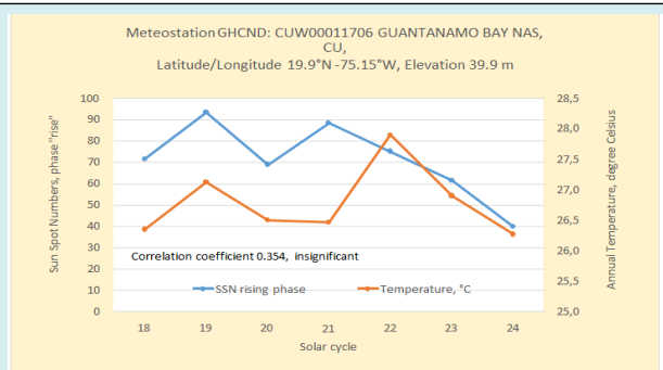
Figure 13: There is no statistically significant correlation between the mean surface air temperature for the weather station GUANTANAMO BAY NAS, CUBA, and the mean sunspot number during the phase “rise” of the 7 solar activity cycles (for which data are available).
