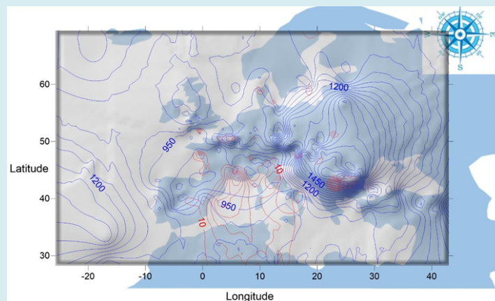
Figure 20: The main areas of influence of solar alpha radiation on mortality in the Europe and Mediterranean region are the Balkans and, to a lesser extent, the Western Mediterranean. (Software Surfer 10).
