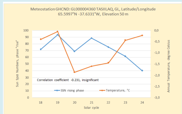
Figure 12: There is no statistically significant correlation between the mean surface air temperature for weather station TASIILAQ, GREENLAND, and the mean sunspot number during the phase “rise” of the 7 solar activity cycles (for which data are available).
