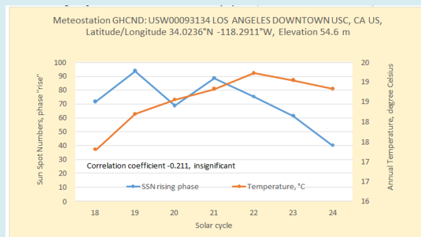
Figure 14: There is no statistically significant correlation between the mean surface air temperature for the weather station LOS ANGELES DOWNTOWN USC, USA, and the mean sunspot number during the phase “rise” of the 7 cycles of solar activity (for which data are available).
