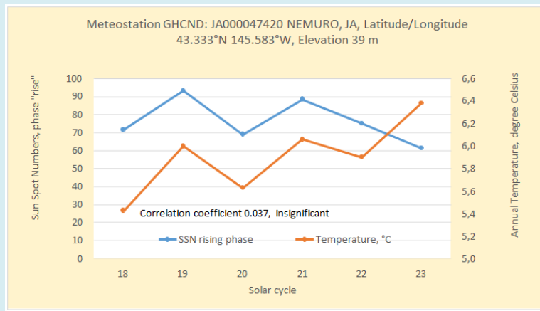
Figure 17: There is no statistically significant correlation between the mean surface air temperature for the NEMURO, JAPAN weather station, and the mean sunspot number during the phase “rise” of the 6 solar activity cycles (for which data are available).
