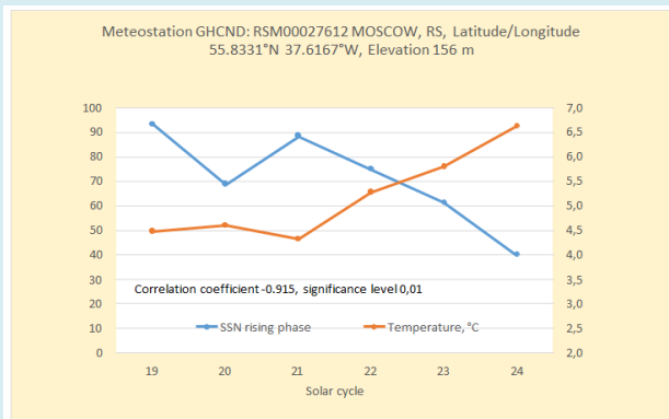
Figure 11: There is a high statistically significant negative correlation between the mean surface air temperature for weather station MOSCOW, RUSSIA, and the mean sunspot number during the phase “rise” of the 6 solar activity cycles (for which data are available).
